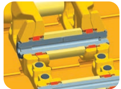
Bagues rotatives
